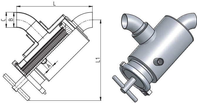
53431-H Dirt trap direct S - S
