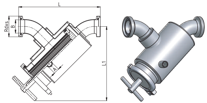
53432-H Dirt trap direct G - G
