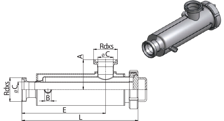
53510-H Corner filter G - G
